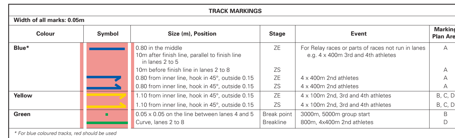
Figure 2.2.1.6a - Marking plan for the 400m Standard Track
